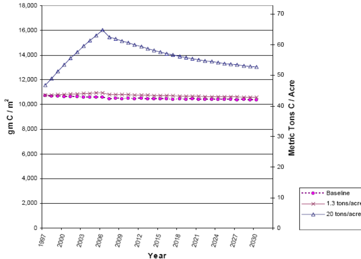
Exhibit 4-3 Total Soil C; Iowa Site, Corn Harvested for Grain
